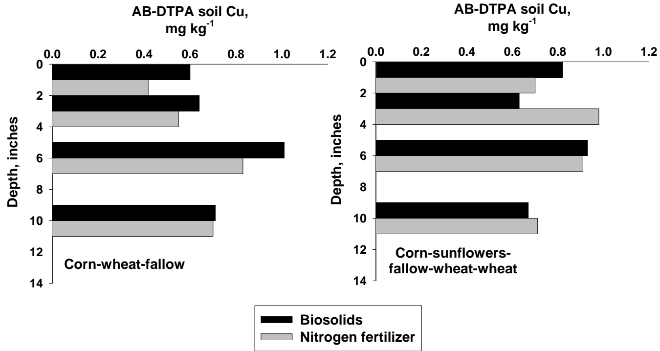
Figure 13. Soil AB-DTPA-extractable Cu concentration for 2002 dryland corn rotations comparing Littleton/Englewood biosolids to commercial N fertilizer. In the statistical summary, LSD_{0.10} represents the least significant difference at the 10% probability level and NS indicates non-significant differences.
