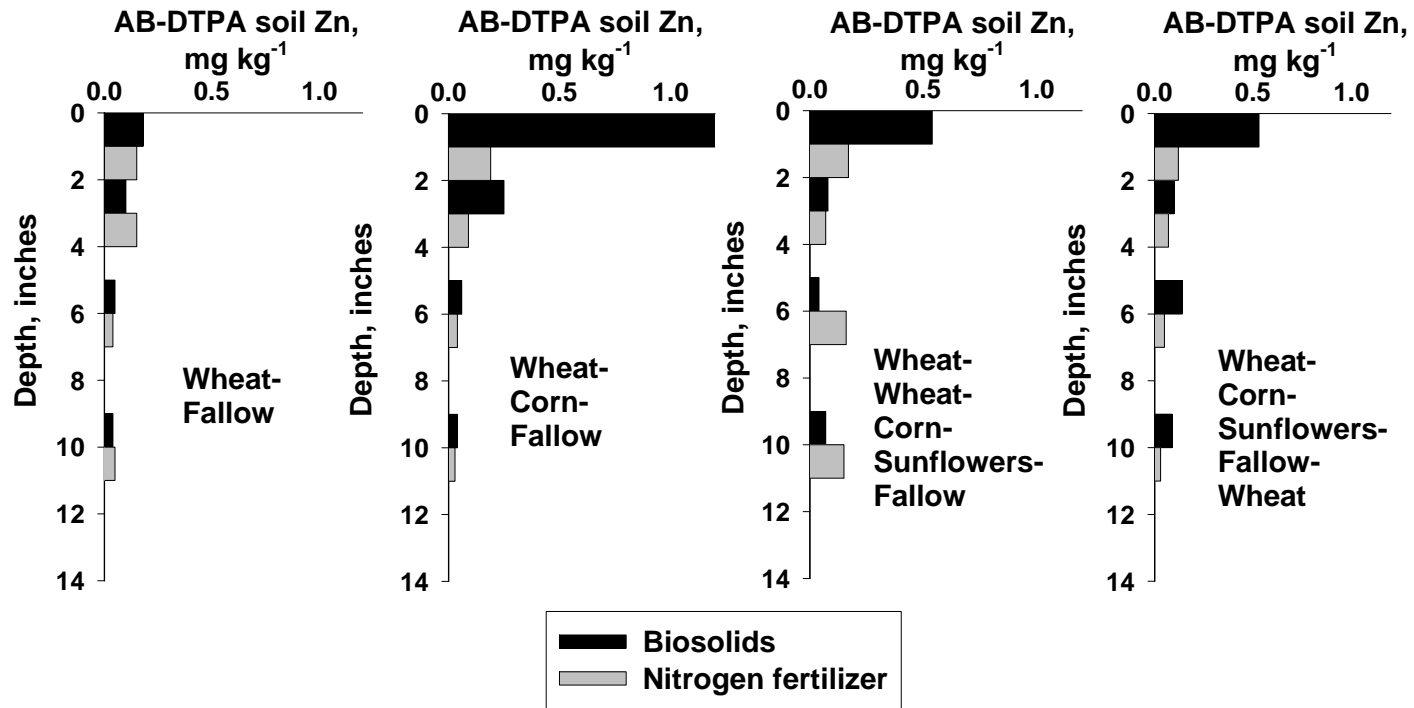
Figure 7. Soil AB-DTPA-extractable Zn concentration following 2022 dryland-wheat-rotation harvests comparing Littleton/Englewood biosolids to commercial N fertilizer. In the statistical summary, LSD_{0.10} represents the least significant difference at the 10% probability level and NS indicates non-significant differences.
