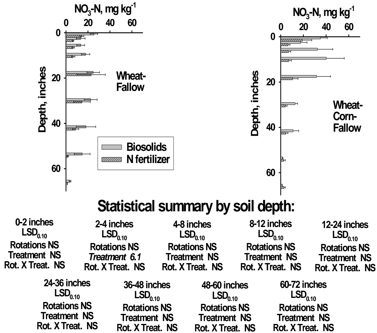
Figure 11. Soil NO 3 -N concentrations following 2007 dryland-wheat-rotation harvests comparing Littleton/Englewood biosolids to commercial N fertilizer. In the statistical summary, LSD 0.10 represents the least significant difference at the 0.10 probability level and NS indicates non-significant differences.
