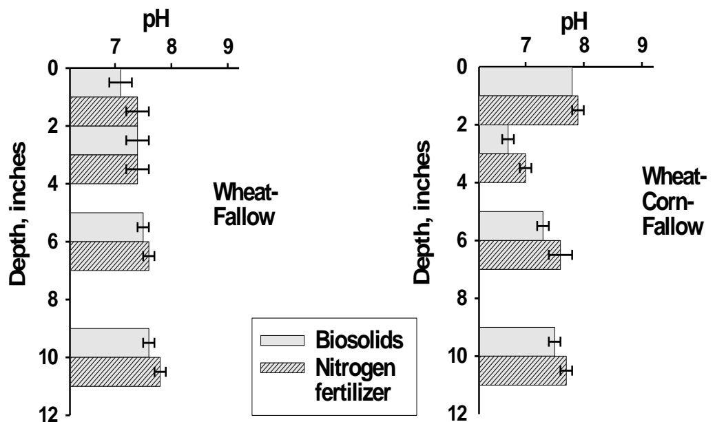
Figure 10. Soil saturated-paste pH following 2007 dryland-wheat-rotation harvests comparing Littleton/Englewood biosolids to commercial N fertilizer. In the statistical summary, LSD_{0.10} represents the least significant difference at the 0.10 probability level and NS indicates non-significant differences.
