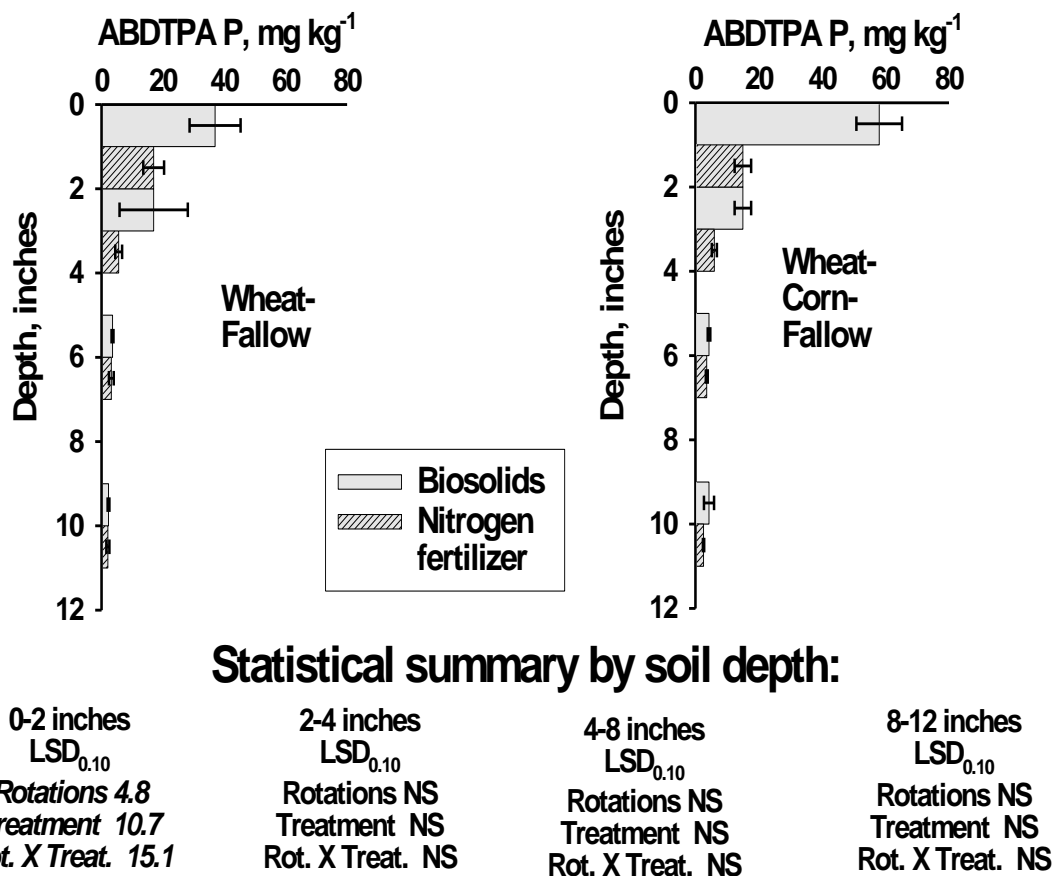
Figure 6. Soil AB-DTPA-extractable P concentration following 2007 dryland-wheat-rotation harvests comparing Littleton/Englewood biosolids to commercial N fertilizer. In the statistical summary, LSD_{0.10} represents the least significant difference at the 0.10 probability level and NS indicates non-significant differences.
