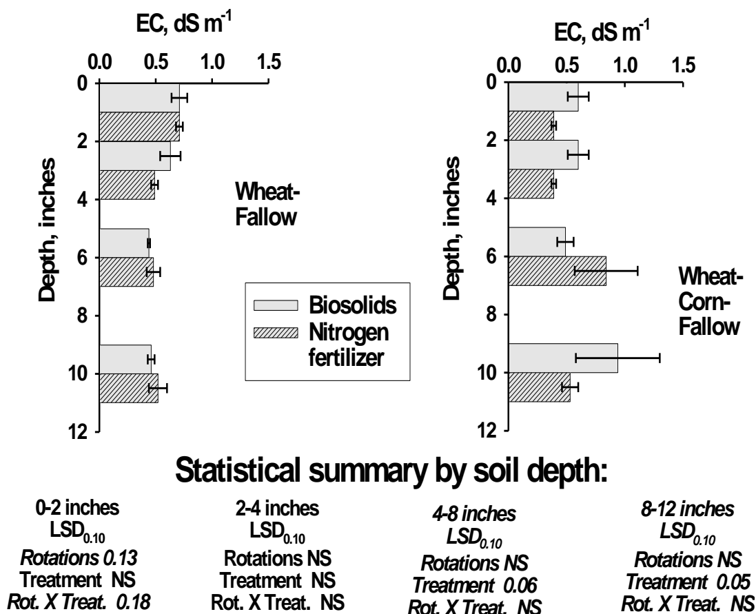
Figure 9. Soil saturated-paste electrical conductivity (EC) following 2007 dryland-wheat-rotation harvests comparing Littleton/Englewood biosolids to commercial N fertilizer. In the statistical summary, LSD_{0.10} represents the least significant difference at the 0.10 probability level and NS indicates non-significant differences.
