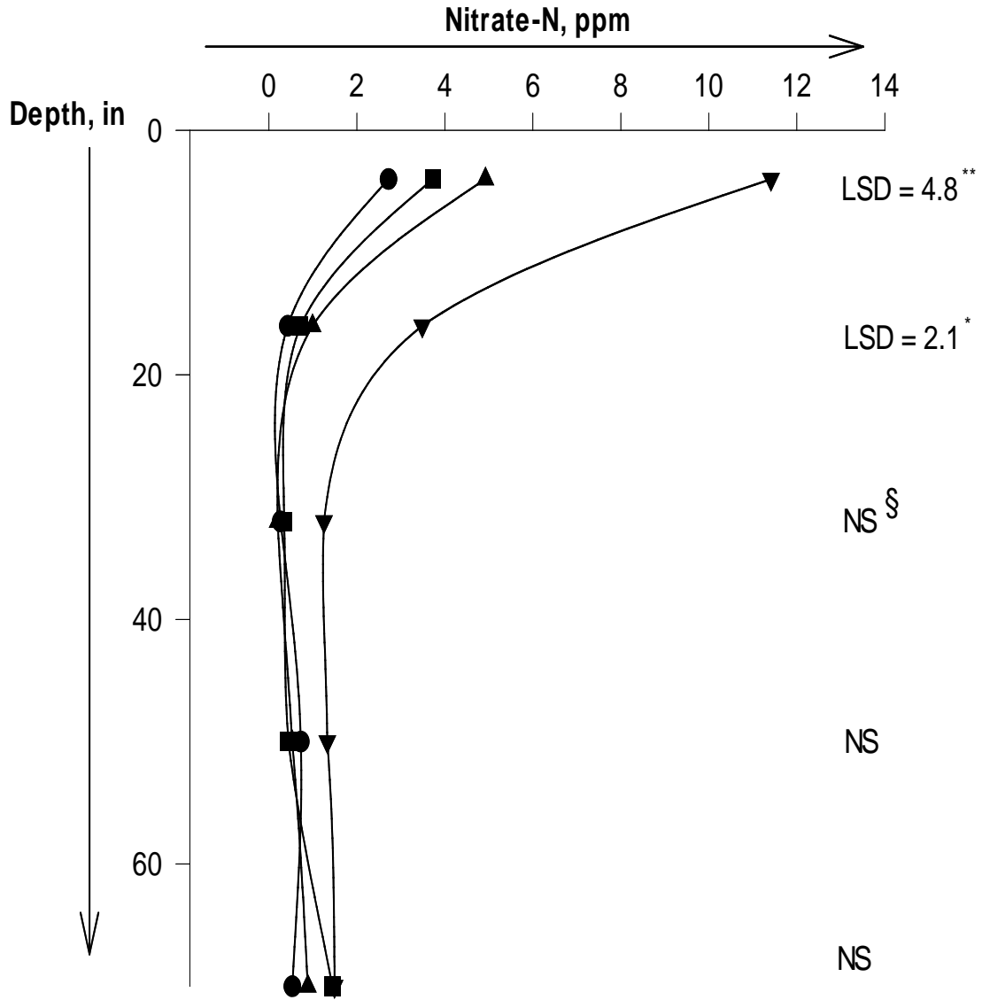
Figure 2. North Bennett Harvest Soil Nitrogen 2000-01.
